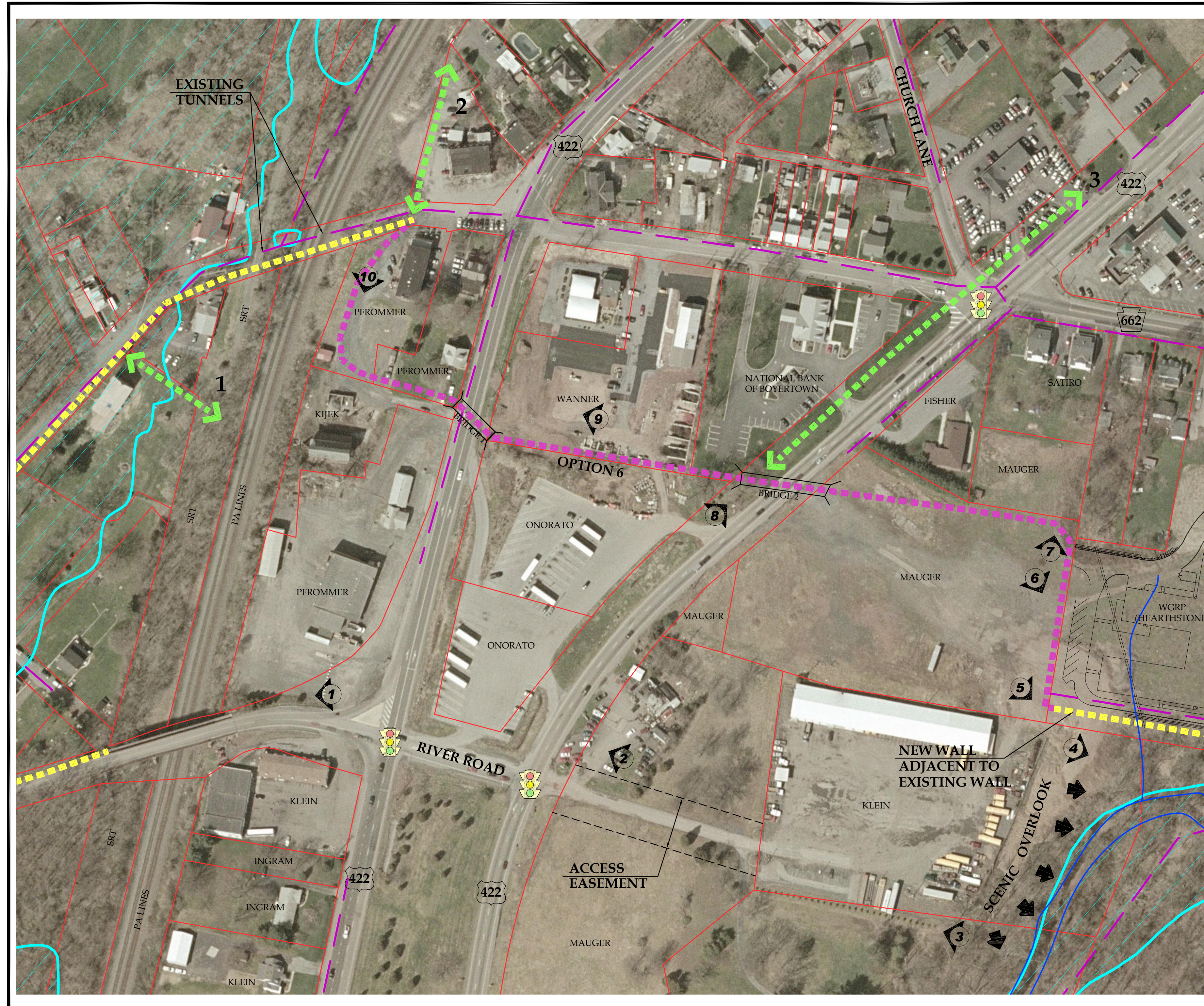
OPTION 6 (TWO BRIDGE CROSSINGS) Approximately 0.3 Miles
